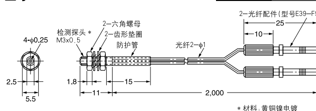
型号E32-D21 (Free)
