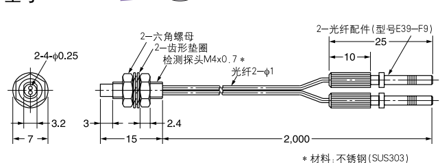
型号E32-D21B NEW (Free)
