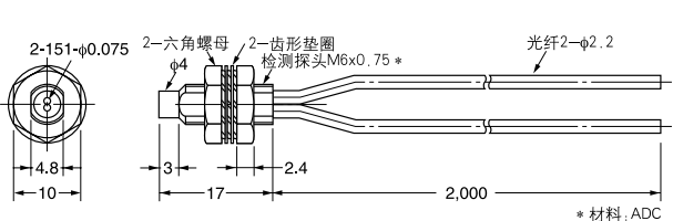
型号E32-D11 (Free)
