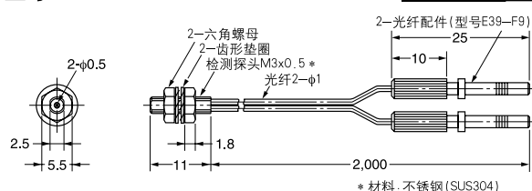
型号E32-DC200F (Free)
