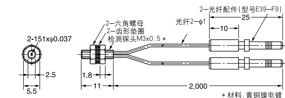
型号E32-D21 (Free)
